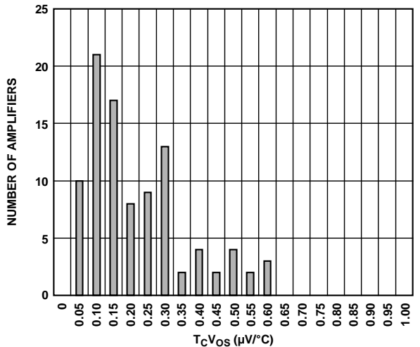
Figure 5. T_C V_{Os}
